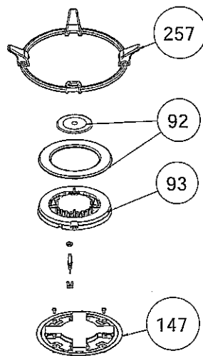
WOK BURNER (OPTIONAL)
