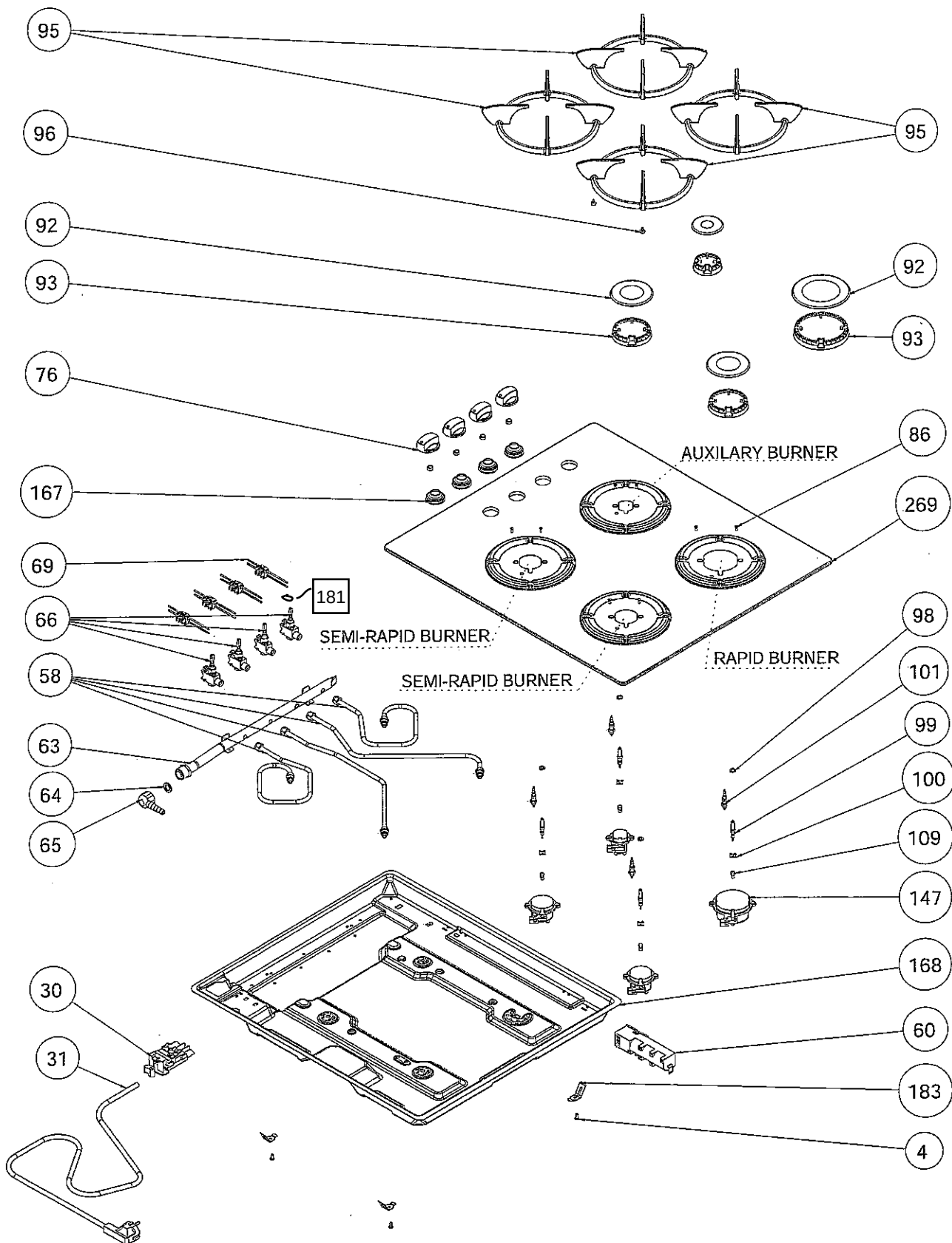
EXPLODED VIEW - SERIE 2 (MODIFIED) GAS-ON-GLASS HOB ASSEMBLY ( AFTER 2011 )
